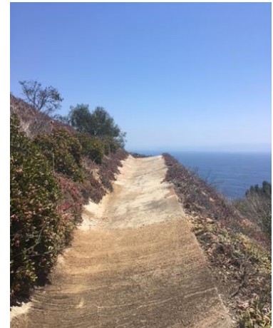
Figure 2 Compliant Swale
