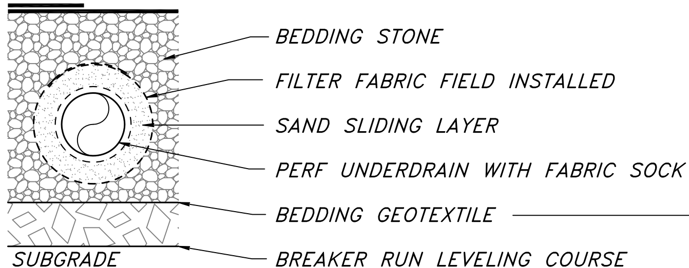
LAPPED LINER
