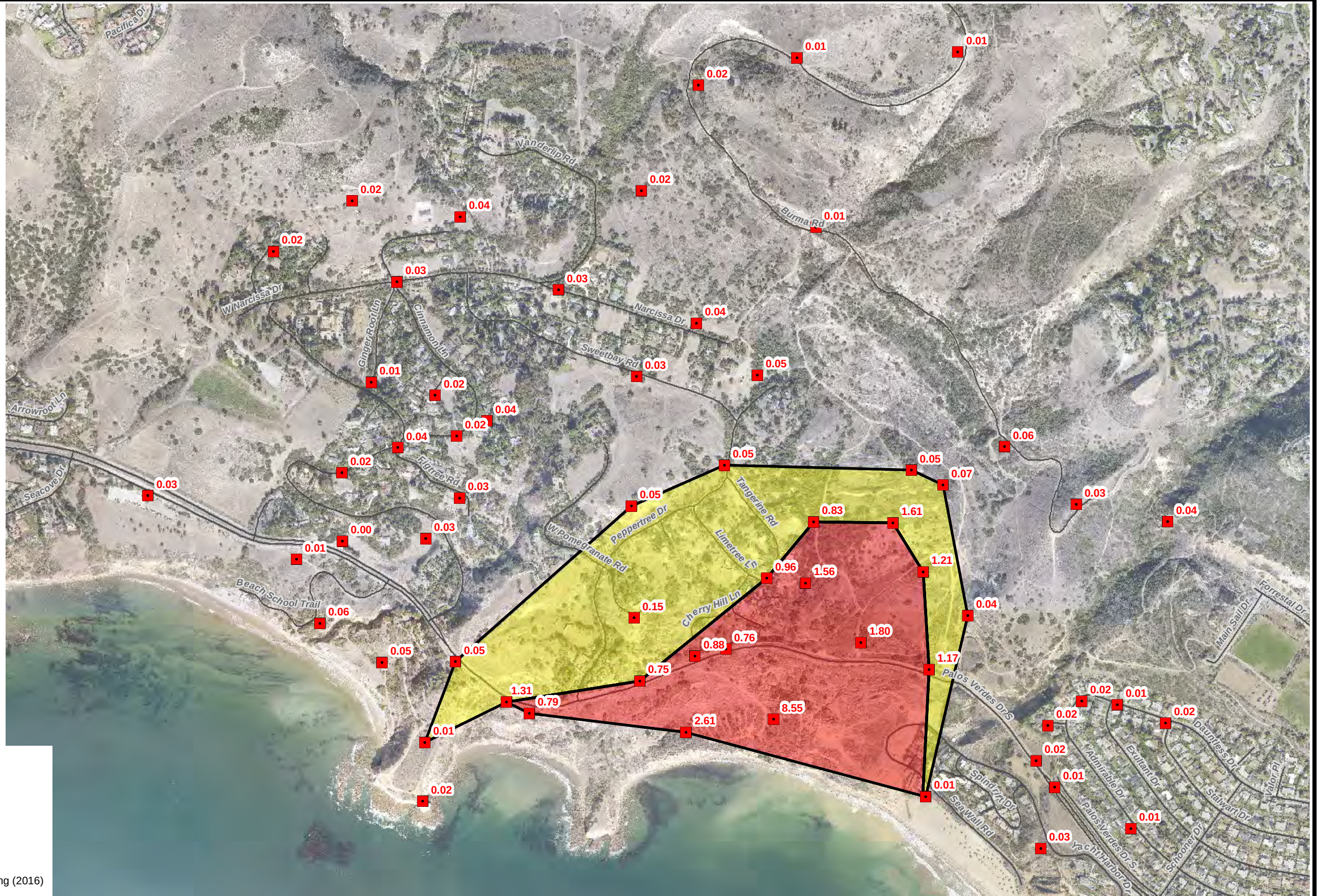
CITY OF RANCHO PALOS VERDES Measured Horizontal Movement 2013-2014
