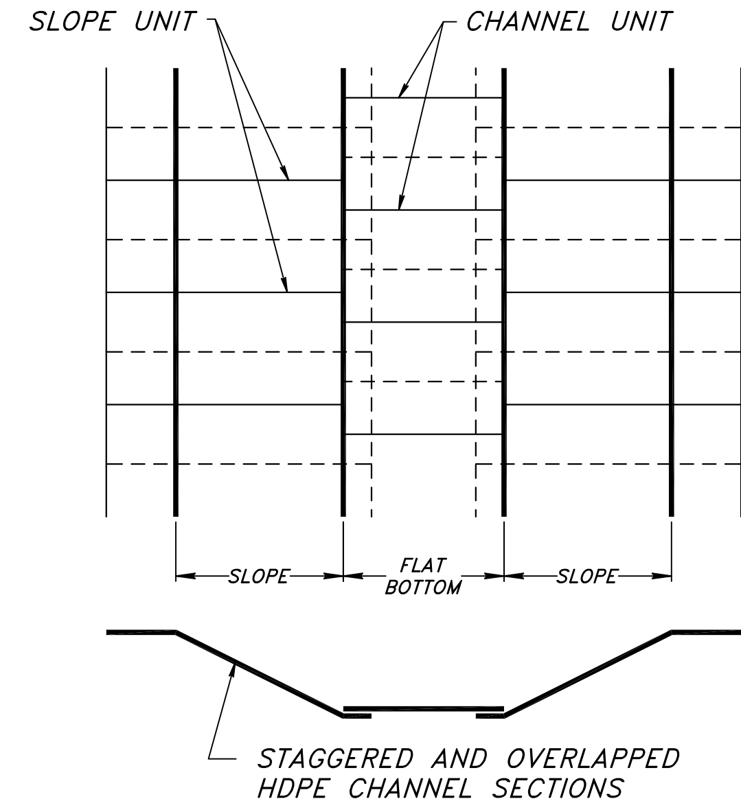
ALTERNATE LAPPED HDPE SECTIONS
