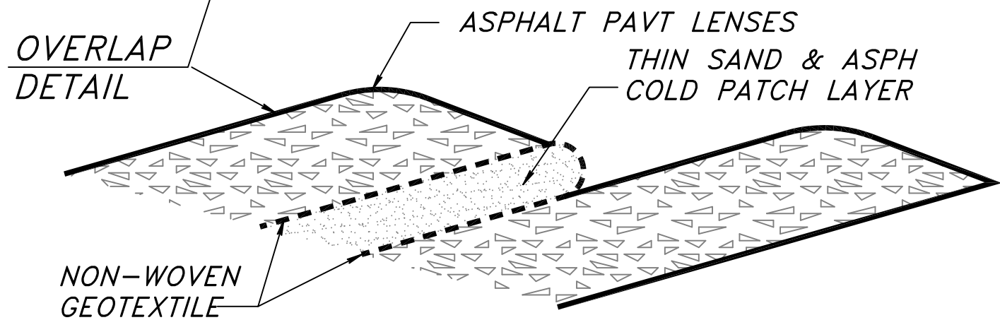
ALTERNATE - LAPPED ASPHALT LENSES
