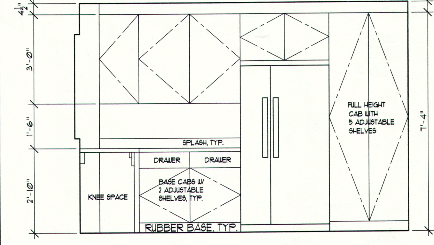
WEST KITCHEN ELEV
