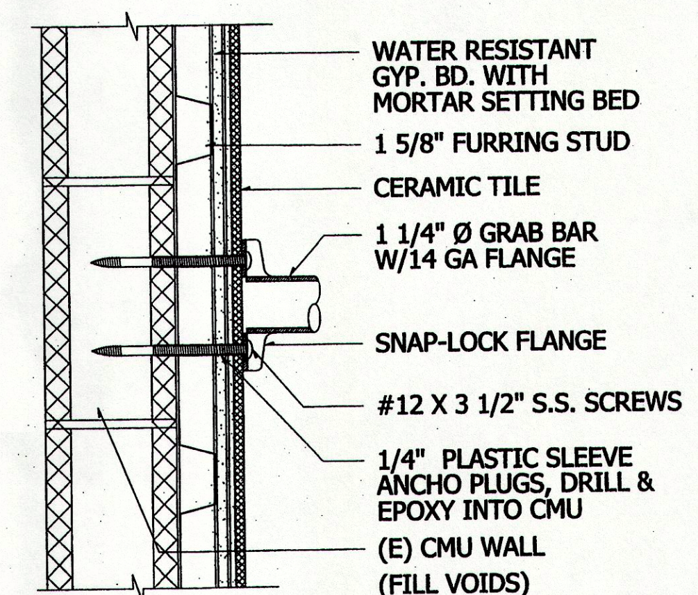
2 TOILET GRAB BAR DETAIL AT CERAMIC TILE/STUD WALLS SCALE 3" = 1'-0"
