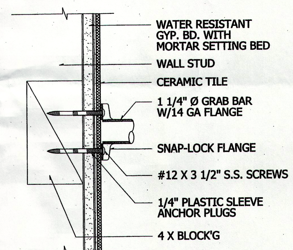
1 TOILET GRAB BAR DETAIL AT CERAMIC TILE/STUD WALLS SCALE 3" = 1'-0"
