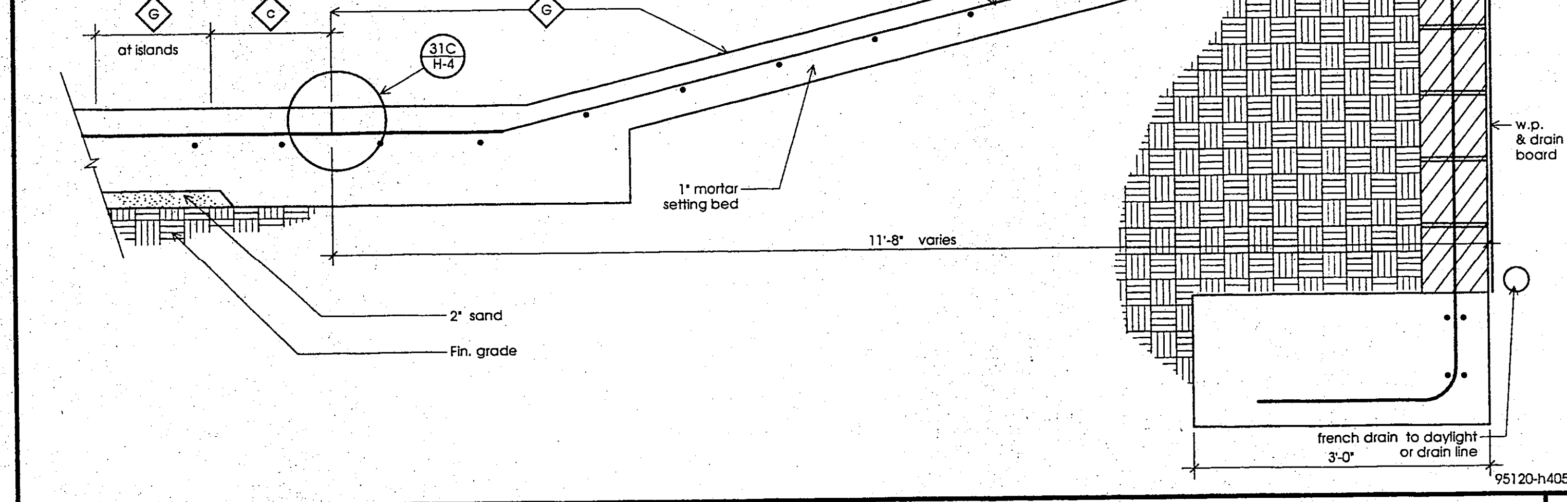
CONCRETE SLOPED PAVING AT "ALASKA" (deduct alternate) Scale: 1" = 1'-0" 21
