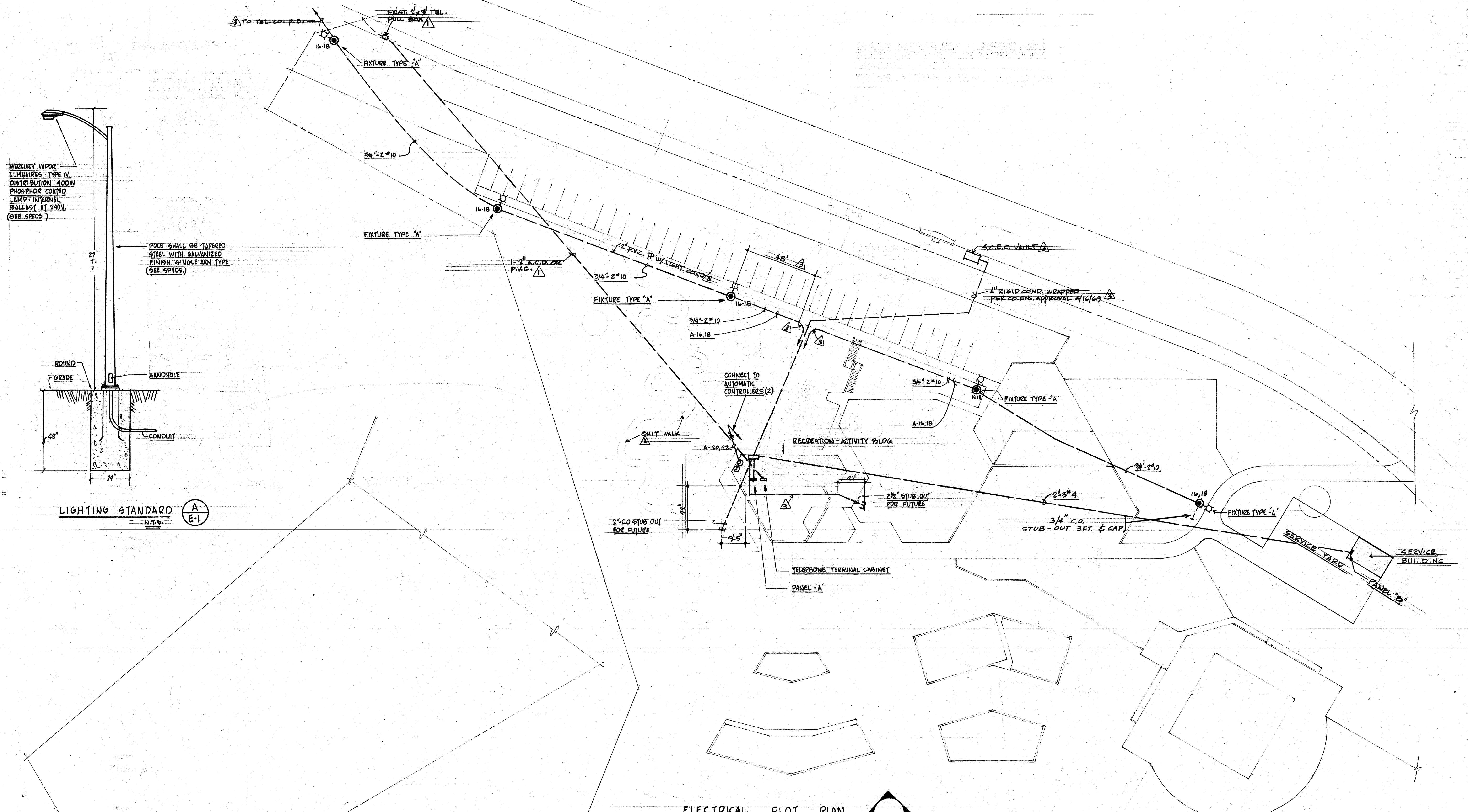
ELECTRICAL PLOT PLAN SCALE: 1/4" = 30'-0"
